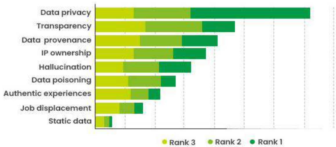
Fig 11: AI ethics [30]
